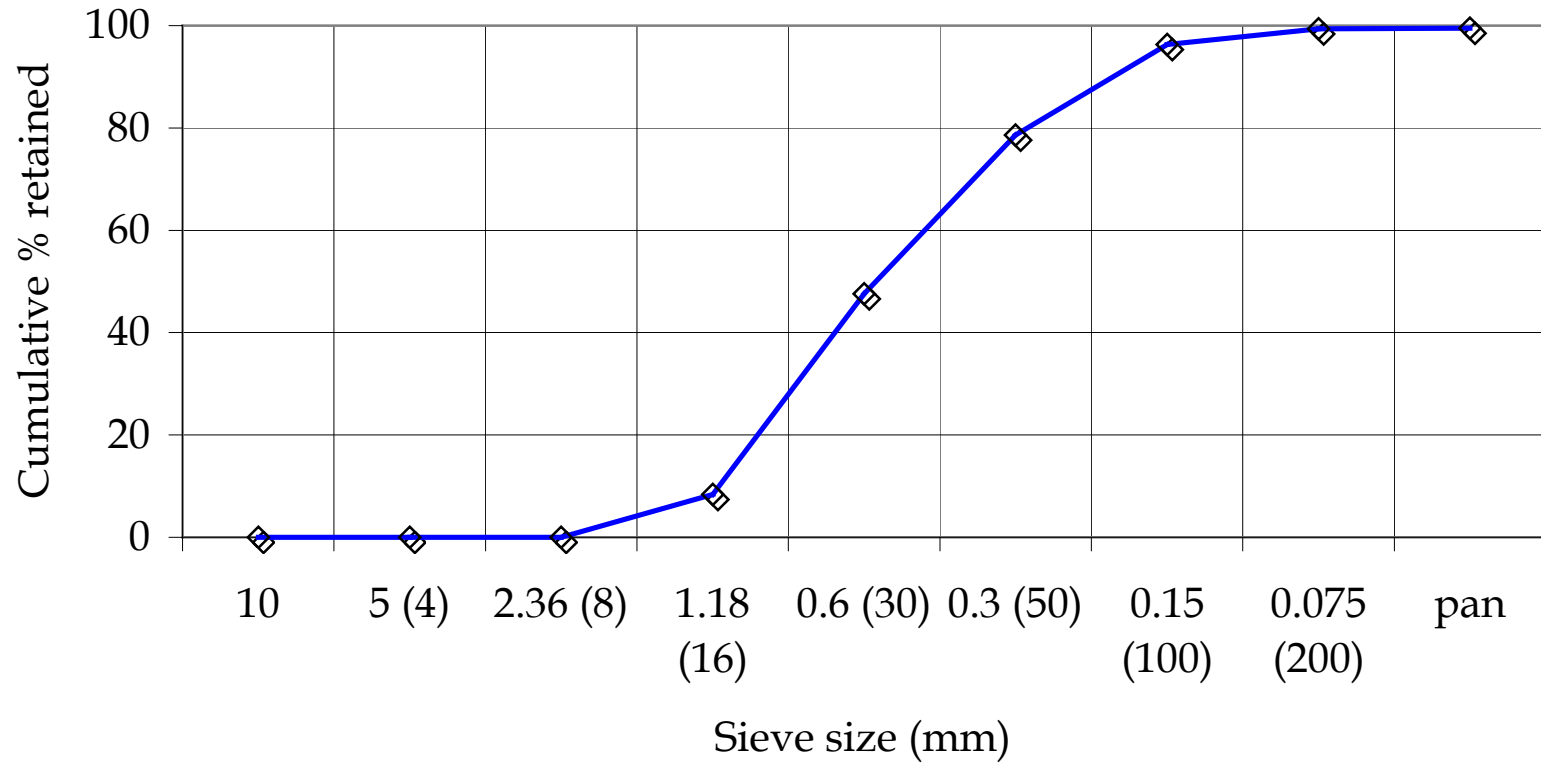
cumulative sand grading curve
